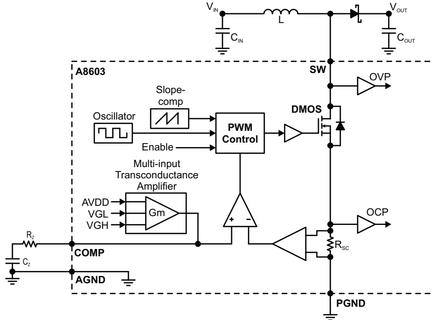
Figure 8: Boost Controller Circuit
