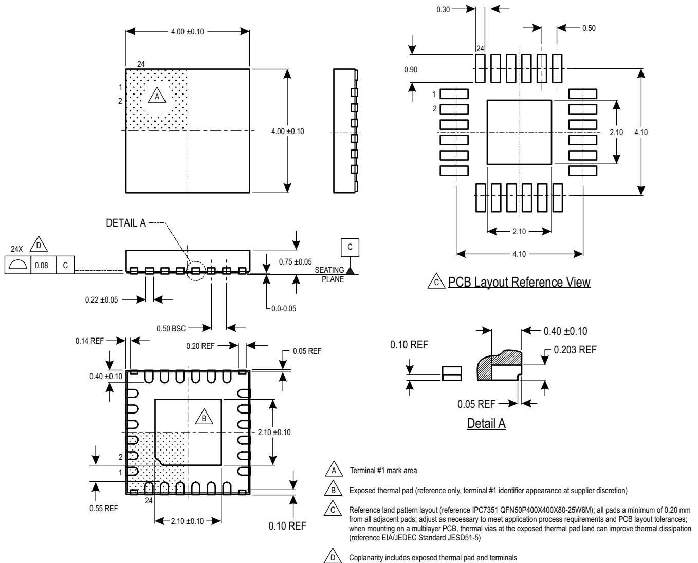
Figure 21: Package ES, 24-Pin 4 mm x 4 mm QFN with Exposed Thermal Pad and Wettable Flank
