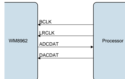
Figure 39 Slave Mode
