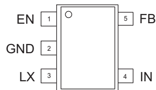
TSOT23-5 (Top View)
