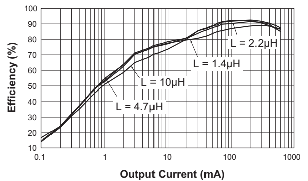
Efficiency vs. Output Current ( V_{IN} = 3.6V ; V_{OUT} = 1.8V ; T_A = 25^\circ C )
