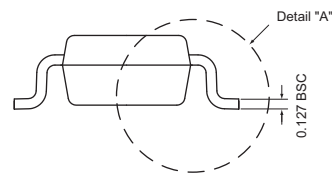
End View
