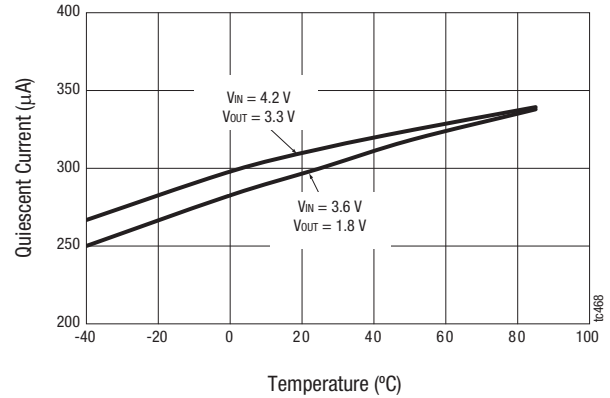
Figure 12. Quiescent Current vs Temperature (L = 2.2 μH, CIN = COUT = 22 μF)
