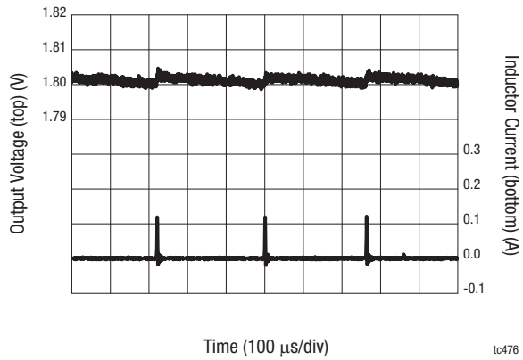
Figure 20. Output Ripple ( V_{IN} = 3.6\text{ V} , V_{OUT} = 1.8\text{ V} , I_{OUT} = 0\text{ A} , L = 2.2\text{ }\mu\text{H} )
