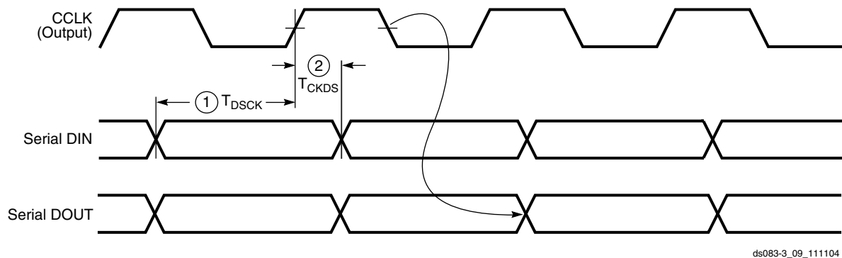
Figure 4: Master Serial Mode Timing Sequence
