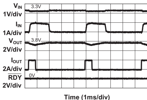
Figure 1: AAT1219 Operation Waveform When 2A 577 \mu s Load Pulse is Applied.
