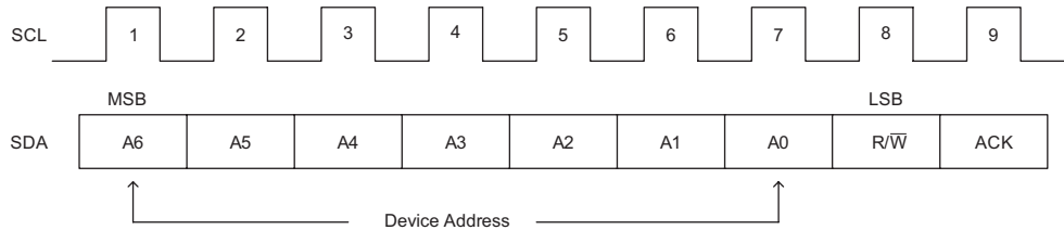
Figure 3: I²C Device Address Bit; 7-bit Slave Address (A6-A0), 1-bit Read/Write (R/W), 1-bit Acknowledge (ACK).
