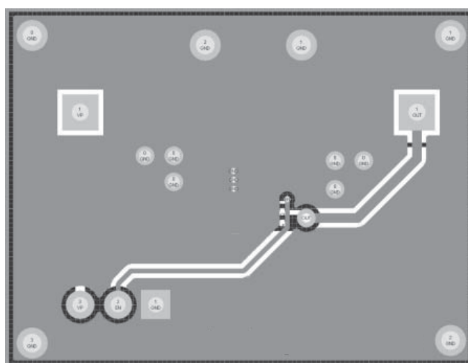
Figure 7: AAT2113B Evaluation Board
