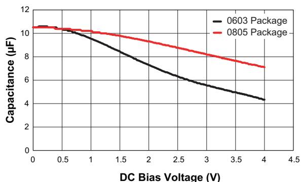
Figure 1: 10 \mu F Capacitor Value vs. DC Bias Voltage for Different Package Sizes.
