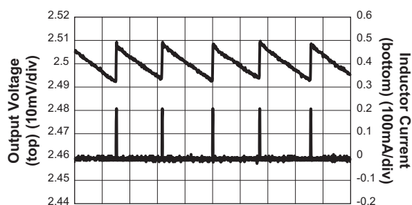
Output Voltage Ripple ( V_{OUT} = 2.5V ; V_{IN} = 3.3V ; I_{OUT} = 1mA )
