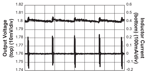
Output Voltage Ripple ( V_{OUT} = 1.8V ; V_{IN} = 3.3V ; I_{OUT} = 1mA )
