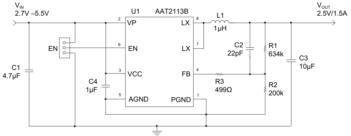
Figure 8: AAT2113B Application Schematic for 2.5V Output Voltage.
