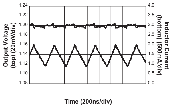
Output Voltage Ripple ( V_{OUT} = 1.2V ; V_{IN} = 3.3V ; I_{OUT} = 1.5A )
