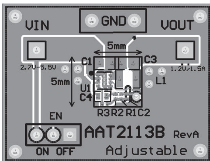
Figure 6: AAT2113B Evaluation Board
