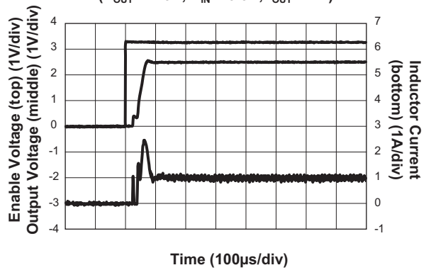
Soft Start ( V_{OUT} = 2.5V ; V_{IN} = 3.3V ; I_{OUT} = 1A )
