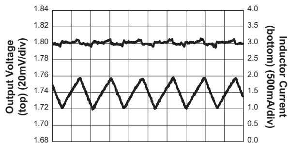
Output Voltage Ripple ( V_{OUT} = 1.8V ; V_{IN} = 3.3V ; I_{OUT} = 1.5A )
