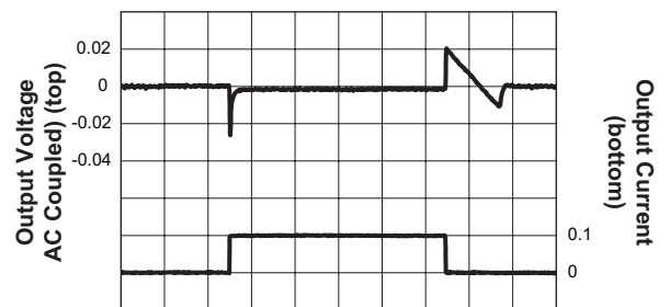
Load Transient
