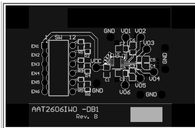
Figure 2: AAT2606 Evaluation Board Top Side Layout.
