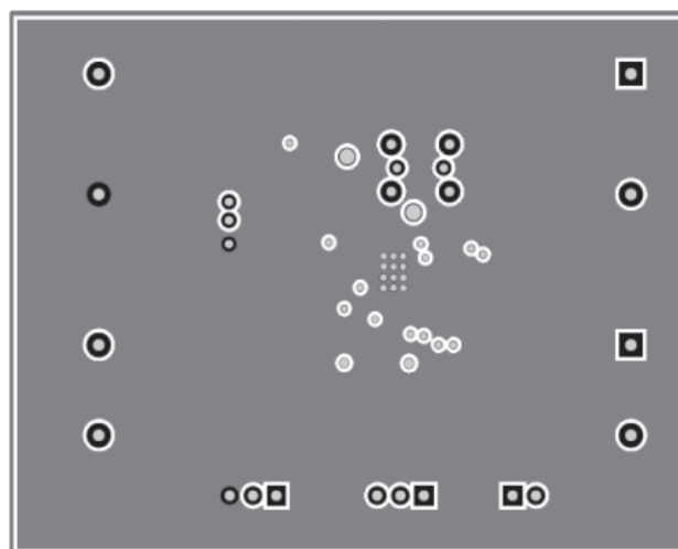
Figure 8: AAT2687IFK Evaluation Board Bottom Layer.
