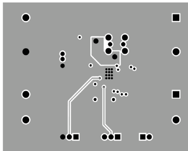
Figure 6: AAT2687IFK Evaluation Board MID1 Layer.
