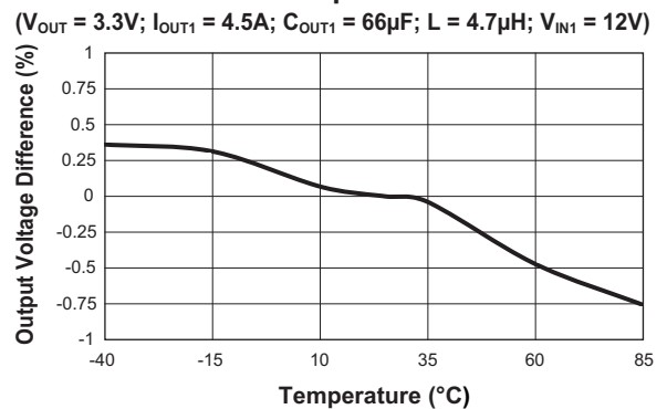
Step-Down Converter Output Voltage vs. Temperature ( V_{OUT} = 3.3V ; I_{OUT1} = 4.5A ; C_{OUT1} = 66µF ; L = 4.7µH ; V_{IN1} = 12V )
