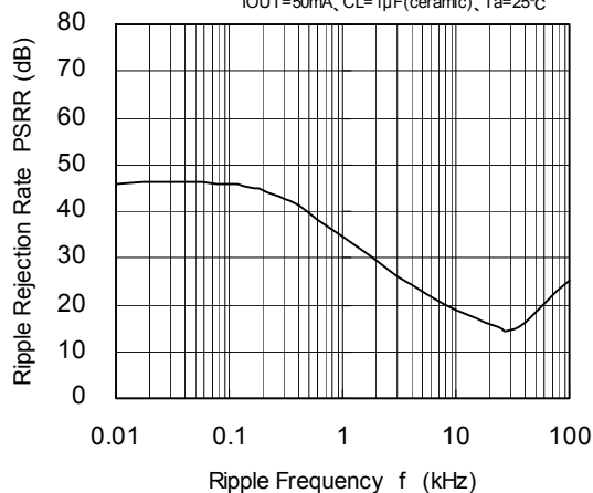
XC6202P332 (3.3V)
