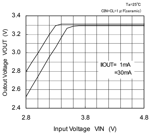
XC6202P332 (3.3V)
