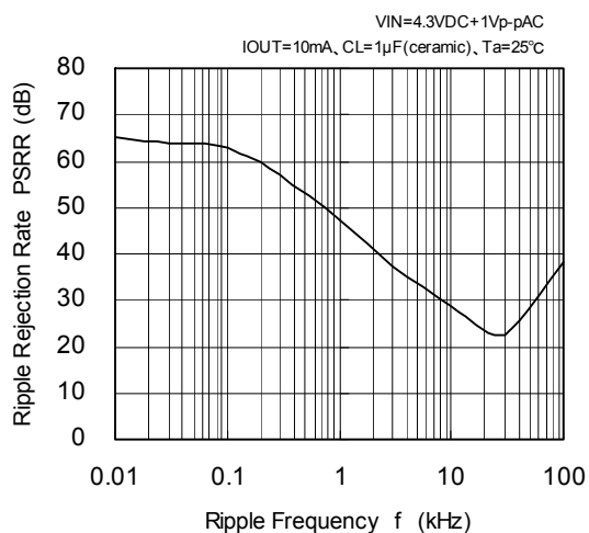
XC6202P332 (3.3V)
