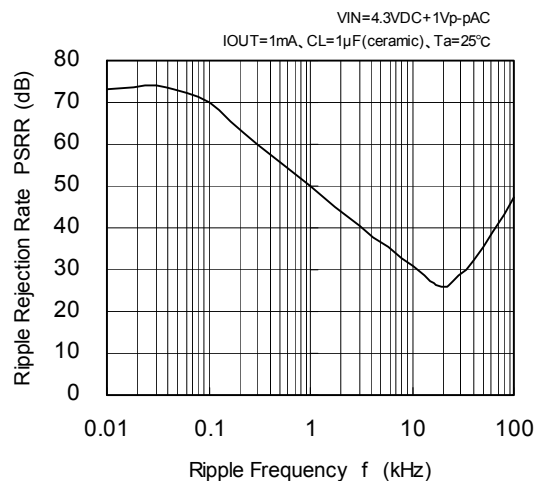
XC6202P332 (3.3V)
