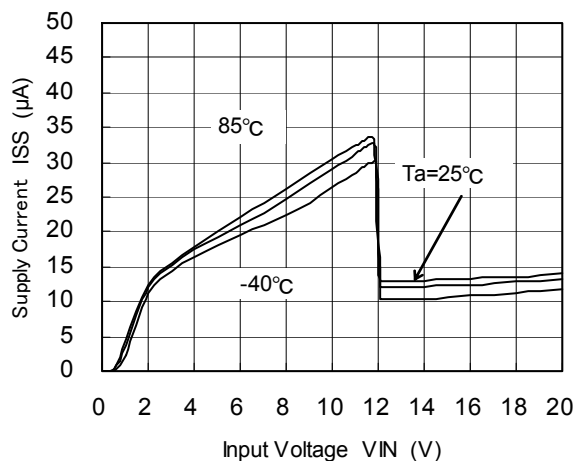
XC6202PC02(12V)
