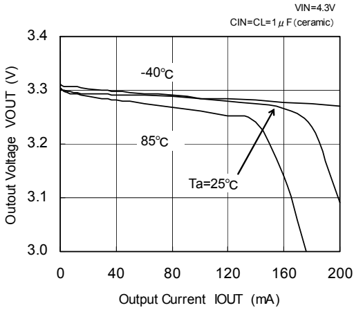
XC6202P332 (3.3V)
