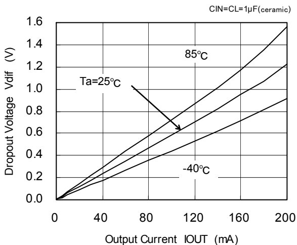
XC6202P332 (3.3V)
