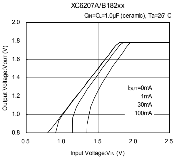
(1) Output Voltage vs. Input Voltage
