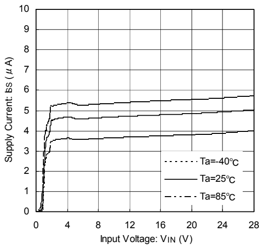
XC6216B/D 332
