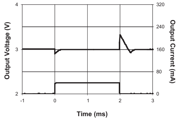
Load Transient – 1mA/40mA
