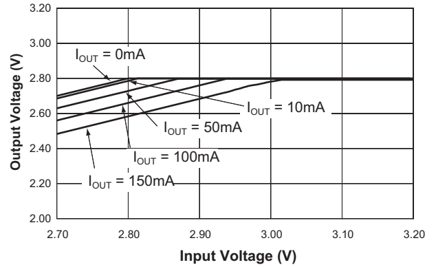
Dropout Characteristics
