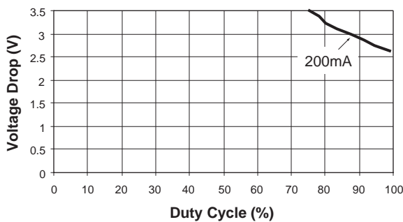
Device Duty Cycle vs. V_{DROP} ( V_{OUT} = 2.5V @ 50°C )
