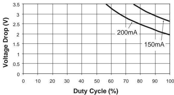
Device Duty Cycle vs. V_{DROP} ( V_{OUT} = 2.5V @ 85°C )
