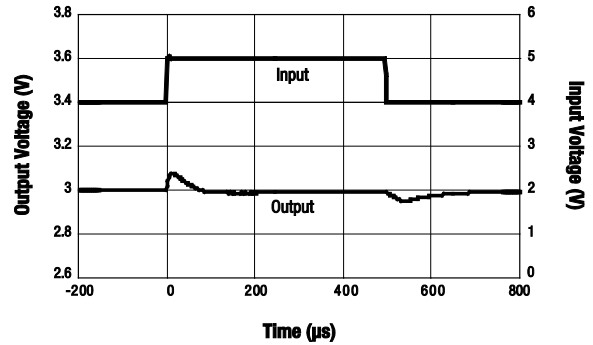
Figure 12. Line Response with 1 mA Load
