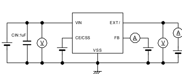
Circuit 4: EXT On Resistance, FB Current
