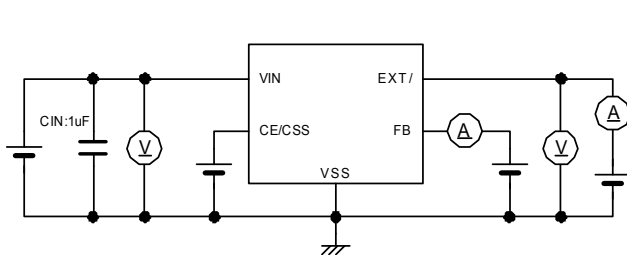
Circuit 4: EXT On Resistance, FB Current
