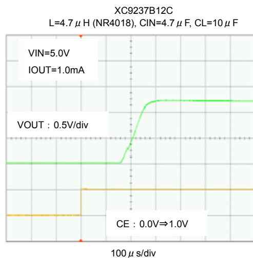
(12) XC9235B/36B/37B Rise Wave Form
