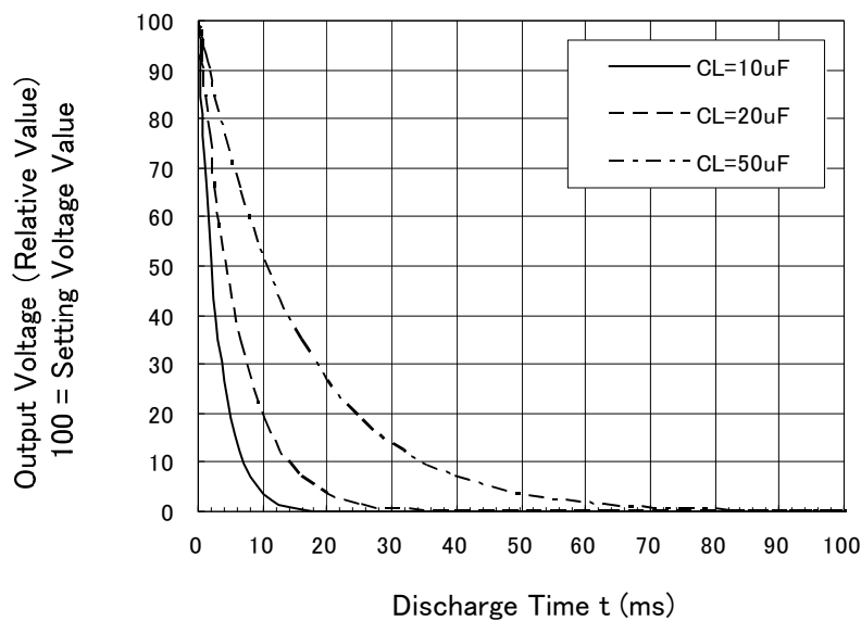
Output Voltage Discharge Characteristics R dischg = 300 \Omega (TYP)
