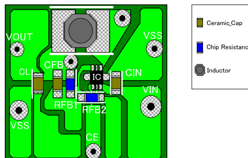
XC9235/XC9236/XC9237 D,F (Output Voltage External Setting) (PKG:USP-6C)
