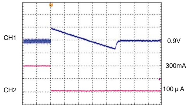
4msec/div CH1: V_{OUT1,2} , AC-COUPLED, 20mV/div CH2: I_{OUT1,2} , 150mA/div
