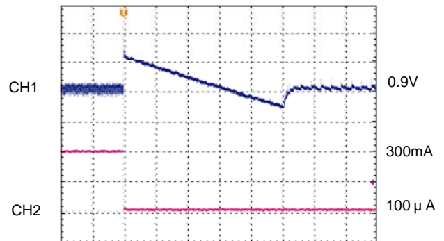
200 \mu sec/div CH1: V_{OUT1,2} , AC-COUPLED, 50mV/div CH2: I_{OUT1,2} , 150mA/div
