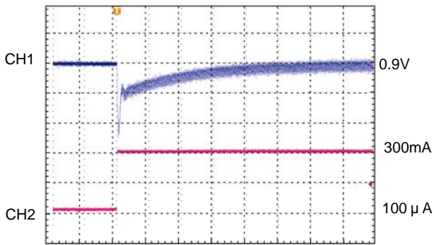
200 \mu sec/div CH1: V_{OUT1,2} , AC-COUPLED, 20mV/div CH2: I_{OUT1,2} , 150mA/div
