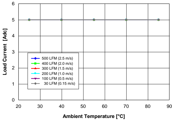
Fig. 1.5V.1: Available load current vs. ambient temperature and airflow rates for V_{out} = 1.5\text{ V} converter mounted vertically with V_{in} = 5\text{ V} , air flowing from pin 5 to pin 1 and maximum MOSFET temperature \leq 120\text{ }^\circ\text{C} .
