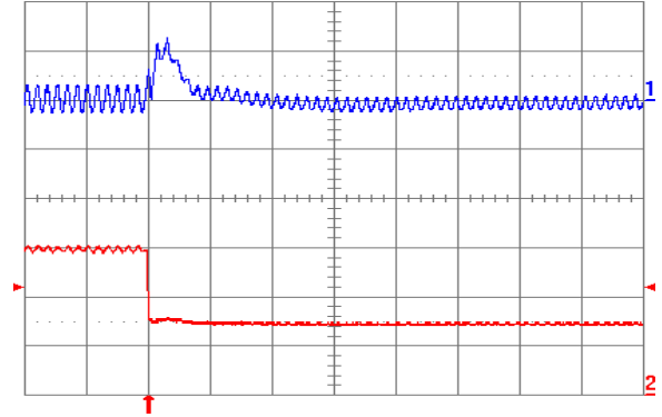
Fig. 1.8V.8: Output voltage response for V_{out} = 1.8\text{ V} to negative load current step change from 5 A to 2.5 A with slew rate of -5\text{ A}/\mu\text{s} at V_{in} = 5\text{ V} . Top trace: output voltage (100 mV/div.); Bottom trace: load current (2 A/div.). C_o = 47\text{ }\mu\text{F} ceramic + 1\text{ }\mu\text{F} ceramic. Time scale: 20\text{ }\mu\text{s}/\text{div} .
