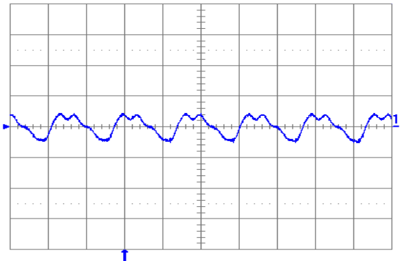
Fig. 2.5V.5: Output voltage ripple (20 mV/div.) at full rated load current into a resistive load with external capacitance 100\text{ }\mu\text{F} ceramic + 1\text{ }\mu\text{F} ceramic and V_{in} = 12\text{ V} for V_{out} = 2.5\text{ V} . Time scale: 2 \mu\text{s} /div.
