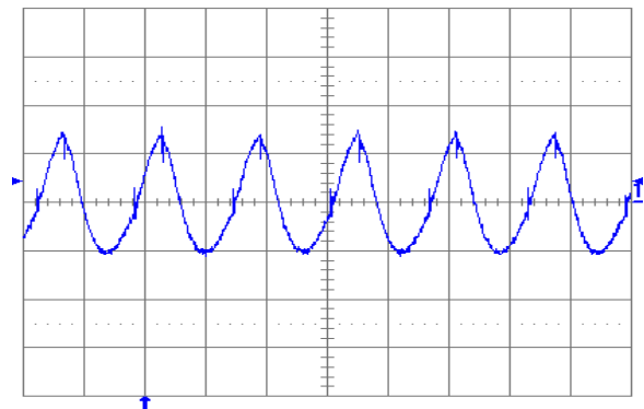
Fig. 1.2V.6: Output voltage ripple (20 mV/div.) at full rated load current into a resistive load with external capacitance 10\ \mu\text{F} ceramic + 1\ \mu\text{F} ceramic and V_{in} = 5\text{ V} for V_{out} = 1.2\text{ V} . Time scale: 2 μs/div.
