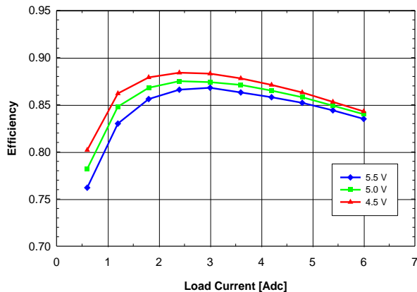
Fig. 1.2V.3: Efficiency vs. load current and input voltage for V_{out} = 1.2\text{ V} converter mounted vertically with air flowing from pin 5 to pin 1 at a rate of 200 LFM (1 m/s) and T_a = 25^\circ\text{C} .
