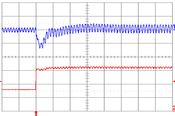
Fig. 2.5V.7: Output voltage response for V_{out} = 2.5\text{ V} to positive load current step change from 3 A to 6 A with slew rate of 5 A/ \mu\text{s} at V_{in} = 5\text{ V} . Top trace: output voltage (100 mV/div.); Bottom trace: load current (2 A/div.). C_o = 47\text{ }\mu\text{F} ceramic + 1 \mu\text{F} ceramic. Time scale: 20 \mu\text{s} /div.
