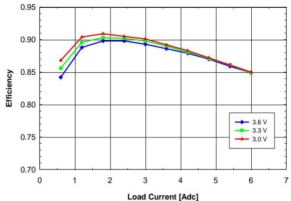
Fig. 1.2V.4: Efficiency vs. load current and input voltage for V_{out} = 1.2\text{ V} converter mounted vertically with air flowing from pin 5 to pin 1 at a rate of 200 LFM (1m/s) and T_a = 25^\circ\text{C} .
