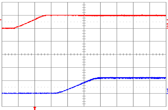
Fig. 1.2V.5: Turn-on transient for V_{out} = 1.2\text{ V} with application of V_{in} at full rated load current (resistive) and 47\ \mu\text{F} external capacitance at V_{in} = 5\text{ V} . Top trace: V_{in} (5 V/div.); Bottom trace: output voltage (1 V/div.); Time scale: 2 ms/div.
