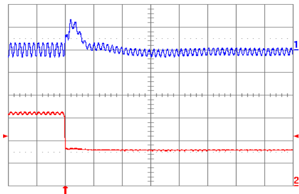
Fig. 2.5V.8: Output voltage response for V_{out} = 2.5\text{ V} to negative load current step change from 6 A to 3 A with slew rate of -5 A/ \mu\text{s} at V_{in} = 5\text{ V} . Top trace: output voltage (100 mV/div.); Bottom trace: load current (2 A/div.). C_o = 47\text{ }\mu\text{F} ceramic + 1 \mu\text{F} ceramic. Time scale: 20 \mu\text{s} /div.
