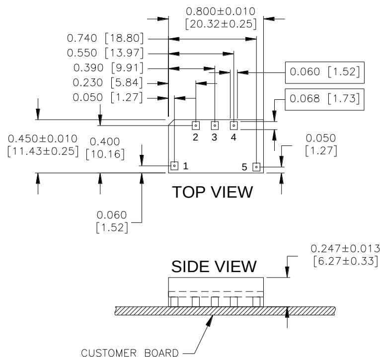
YNM12S Pinout (Surface Mount)
