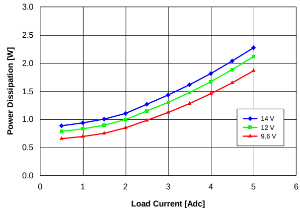
Fig. 3.3V.4: Power Loss vs. load current and input voltage for V_{out} = 3.3 V converter mounted vertically with air flowing at a rate of 200 LFM (1 m/s) and T_a = 25^\circ\text{C} .
