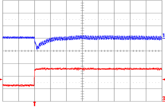
Fig. 5.0V.7: Output voltage response for V_{out} = 5.0 V to positive load current step change from 2.5 A to 5 A with slew rate of 5 \text{ A}/\mu\text{s} at V_{in} = 12 V. Top trace: output voltage (100 mV/div.); Bottom trace: load current (2 A/div.). C_o = 47 \mu\text{F} ceramic. Time scale: 20 \mu\text{s}/\text{div} .
