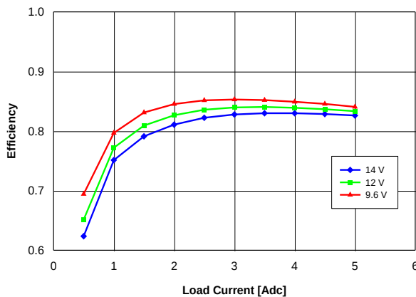
Fig. 1.8V.3: Efficiency vs. load current and input voltage for V_{out} = 1.8 V converter mounted vertically with air flowing at a rate of 200 LFM (1 m/s) and T_a = 25^\circ\text{C} .
