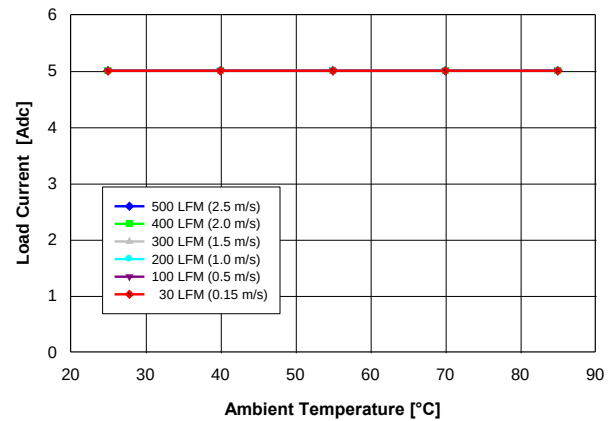
Fig. 1.8V.2: Available load current vs. ambient temperature and airflow rates for V_{out} = 1.8 V converter mounted horizontally with V_{in} = 12 V, and maximum MOSFET temperature \leq 120^\circ\text{C} .
