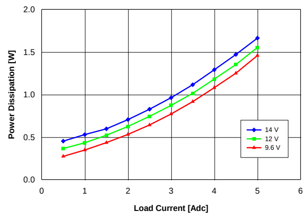
Fig. 1.0V.4: Power Loss vs. load current and input voltage for V_{out} = 1.0 V converter mounted vertically with air flowing at a rate of 200 LFM (1 m/s) and T_a = 25^\circ\text{C} .
