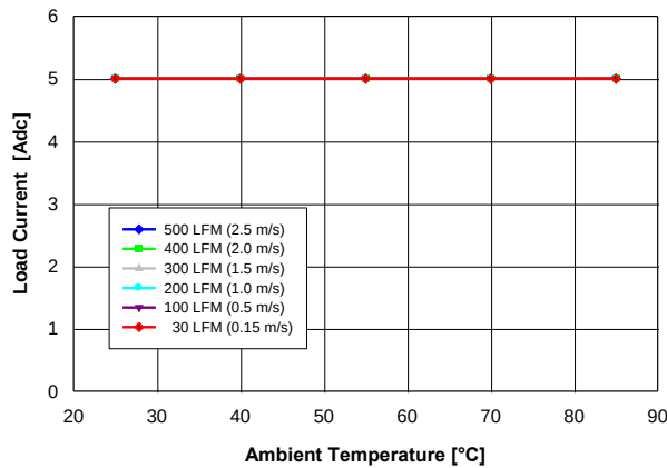
Fig. 1.8V.1: Available load current vs. ambient temperature and airflow rates for V_{out} = 1.8 V converter mounted vertically with V_{in} = 12 V, and maximum MOSFET temperature \leq 120^\circ\text{C} .
