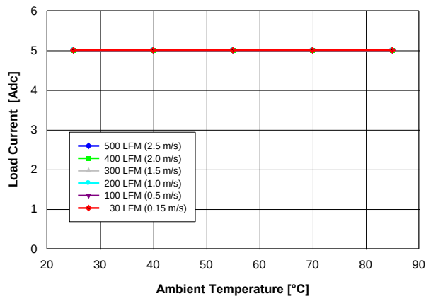
Fig. 1.0V.1: Available load current vs. ambient temperature and airflow rates for V_{out} = 1.0 V converter mounted vertically with V_{in} = 12 V, and maximum MOSFET temperature \leq 120^\circ\text{C} .
