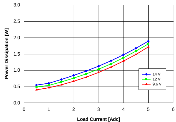
Fig. 1.8V.4: Power Loss vs. load current and input voltage for V_{out} = 1.8 V converter mounted vertically with air flowing at a rate of 200 LFM (1 m/s) and T_a = 25^\circ\text{C} .
