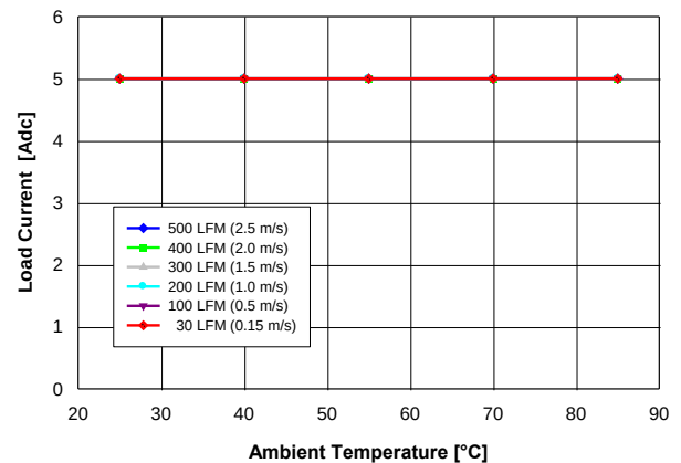
Fig. 1.0V.2: Available load current vs. ambient temperature and airflow rates for V_{out} = 1.0 V converter mounted horizontally with V_{in} = 12 V, and maximum MOSFET temperature \leq 120^\circ\text{C} .
