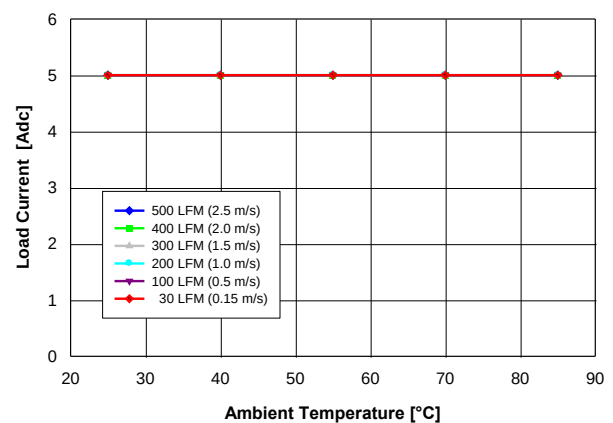
Fig. 2.5V.2: Available load current vs. ambient temperature and airflow rates for V_{out} = 2.5 V converter mounted horizontally with V_{in} = 12 V, and maximum MOSFET temperature \leq 120 ^{\circ} C.
