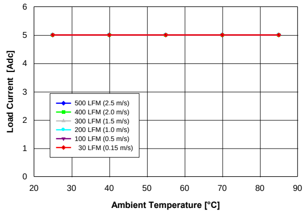
Fig. 3.3V.2: Available load current vs. ambient temperature and airflow rates for V_{out} = 3.3 V converter mounted horizontally with V_{in} = 12 V, and maximum MOSFET temperature \leq 120^\circ\text{C} .
