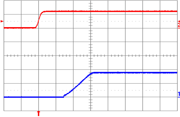
Fig. 1.8V.5: Turn-on transient for V_{out} = 1.8\text{ V} with application of V_{in} at full rated load current (resistive) and 47\text{ }\mu\text{F} external capacitance at V_{in} = 12\text{ V} . Top trace: V_{in} (10 V/div.); Bottom trace: output voltage (1 V/div.); Time scale: 5 ms/div.
