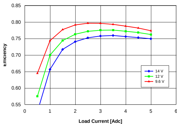
Fig. 1.0V.3: Efficiency vs. load current and input voltage for V_{out} = 1.0 V converter mounted vertically with air flowing at a rate of 200 LFM (1 m/s) and T_a = 25^\circ\text{C} .
