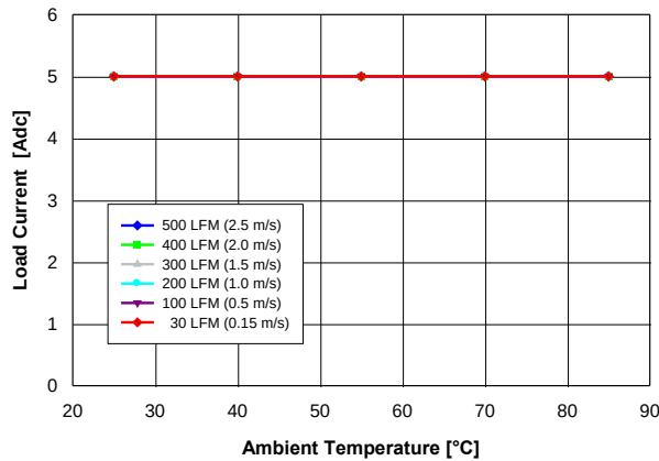
Fig. 3.3V.1: Available load current vs. ambient temperature and airflow rates for V_{out} = 3.3 V converter mounted vertically with V_{in} = 12 V, and maximum MOSFET temperature \leq 120^\circ\text{C} .
