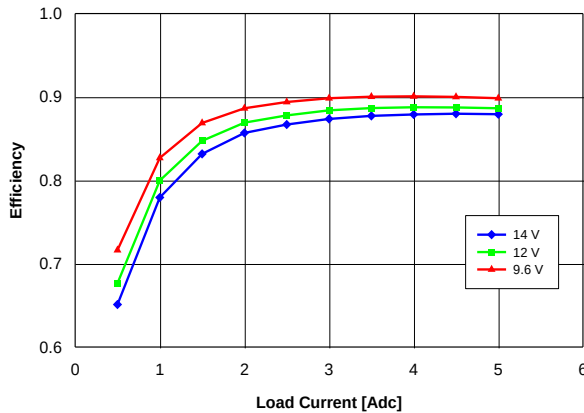
Fig. 3.3V.3: Efficiency vs. load current and input voltage for V_{out} = 3.3 V converter mounted vertically with air flowing at a rate of 200 LFM (1 m/s) and T_a = 25^\circ\text{C} .
