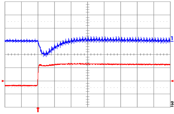
Fig. 2.0V.6: Output voltage response for V_{out} = 2.0 V to positive load current step change from 8 A to 16 A with slew rate of 5 \text{ A}/\mu\text{s} at V_{in} = 12 V. Top trace: output voltage (200 mV/div.); Bottom trace: load current (5 A/div.). C_o = 100 \mu\text{F} ceramic. Time scale: 20 \mu\text{s} /div.
