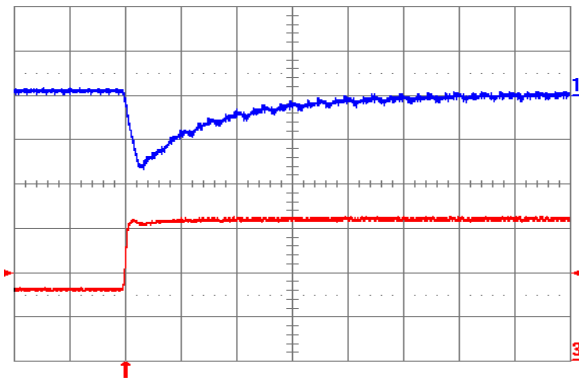
Fig. 1.2V.7: Output voltage response for V_{out} = 1.2\text{ V} to positive load current step change from 8 A to 16 A with slew rate of 5\text{ A}/\mu\text{s} at V_{in} = 5\text{ V} . Top trace: output voltage (100 mV/div.); Bottom trace: load current (5 A/div.). C_o = 100\ \mu\text{F} ceramic. Time scale: 20\ \mu\text{s}/\text{div}
