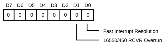
Figure 72. MIMIC Modification Register
