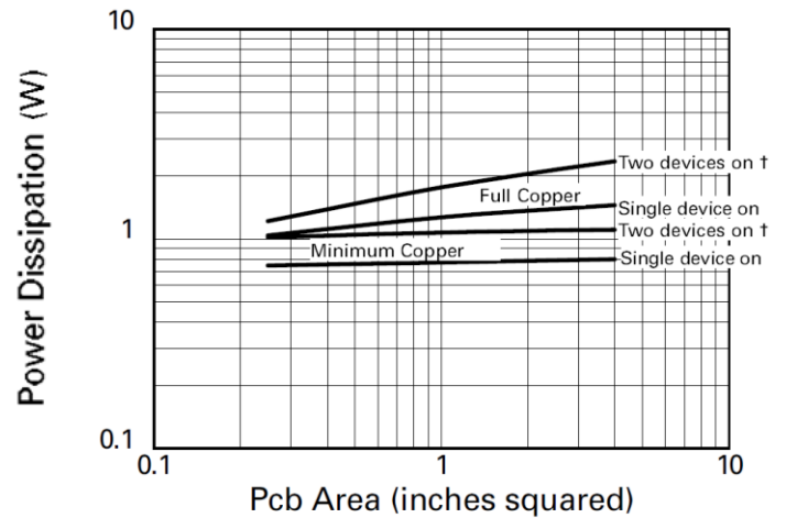
Pd v PCB Area Comparison
