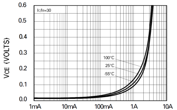
Collector Current
