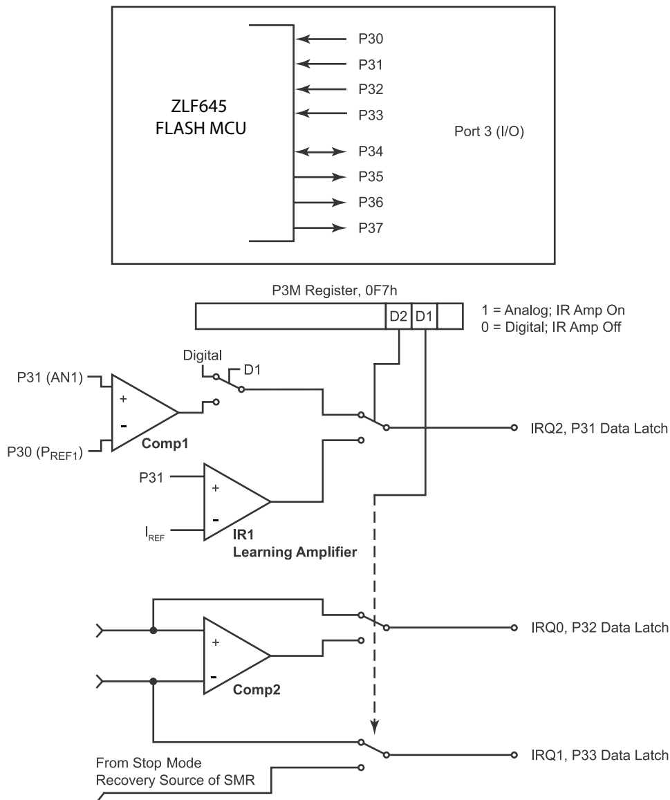
Figure 9. Port 3 Configuration
