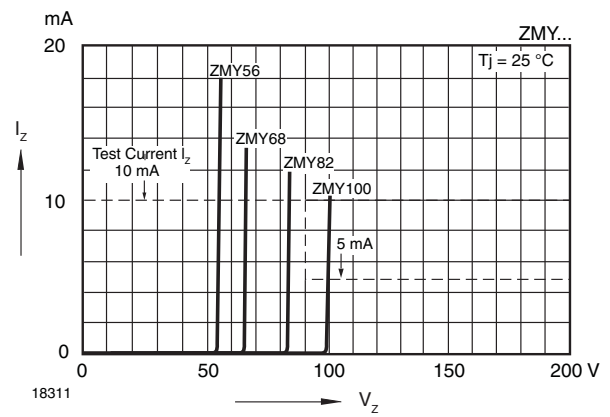
Fig. 8 - Breakdown Characteristics
