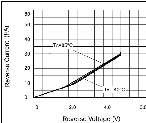
Reverse Characteristics
