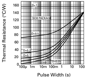
Thermal Resistance v Pulse Width
