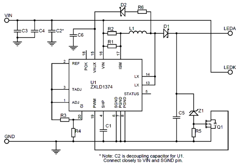
Figure 52 Application Circuit of 350mA Buck-Boost LED Driver
