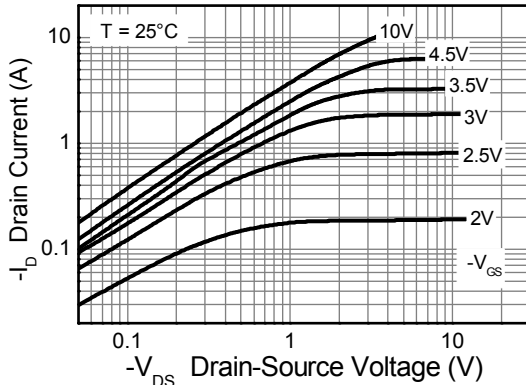
Output Characteristics
