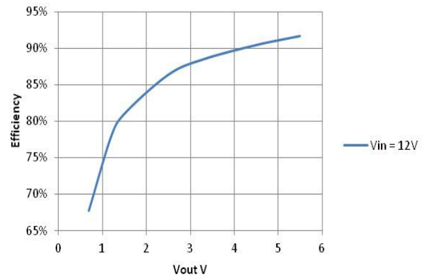
Figure 5. Efficiency vs. Output Voltage, I_{out} = 7\text{A} , F_{sw} = 500\text{kHz}
