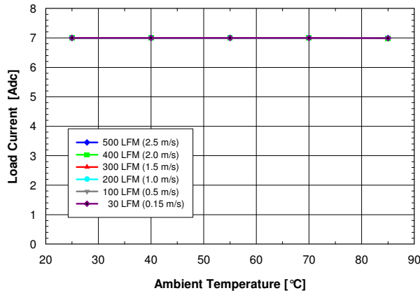
Figure 1. Available output current vs. ambient air temperature and airflow rates for converter DP7010 mounted horizontally with air flowing from input to output, MOSFET temperature \leq 120^\circ\text{C} , V_{in} = 12\text{ V} , V_{out} = 5\text{ V} , and F_{sw} = 500\text{KHz}
