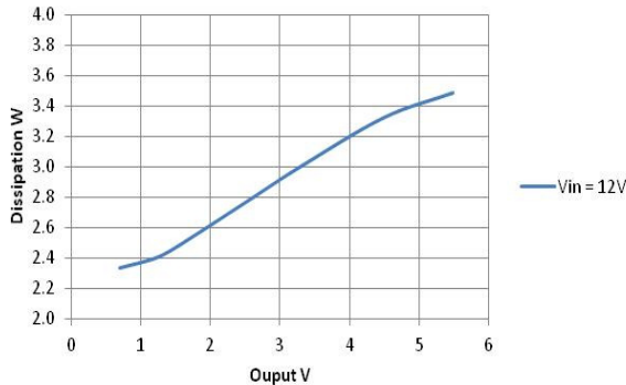
Figure 6. Dissipation vs Voltage. Iout=7A, Fsw=500kHz
