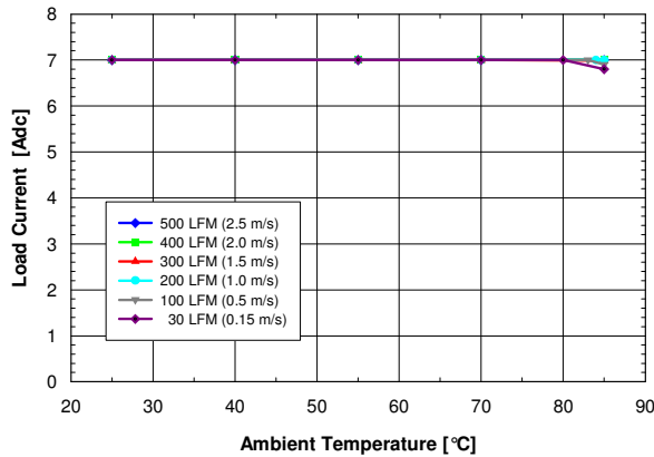
Figure 2. Available output current vs. ambient air temperature and airflow rates for converter DP7010 mounted horizontally with air flowing from input to output, MOSFET temperature \leq 120^\circ\text{C} , V_{in} = 12\text{ V} , V_{out} = 5\text{ V} , and F_{sw} = 1\text{MHz}
