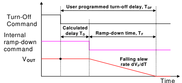
Figure 14. Relationship between Turn-Off Delay and Falling Slew Rate
