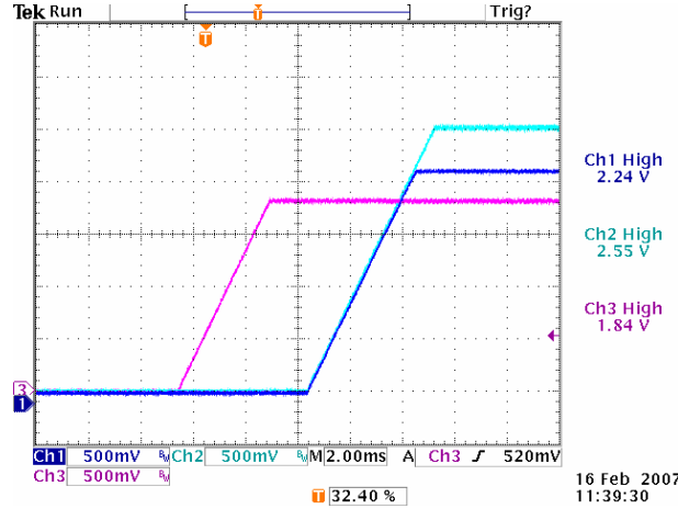
Figure 20 Two outputs delayed 5ms. All slew rates at 0.5V/ms.
