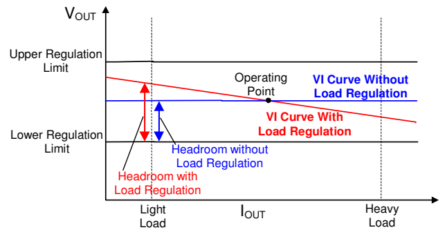
Figure 9. Optimal Voltage Positioning Concept
