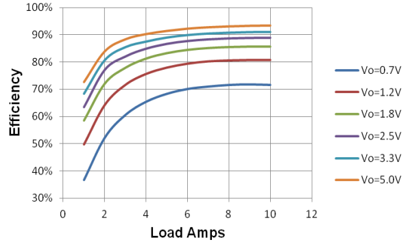
Figure 3. Efficiency vs. Load. V_{in} = 12\text{V} , F_{sw} = 500\text{KHz}
