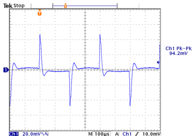
Figure 10 Transient Response with Regulation set to 0 mV/A.
