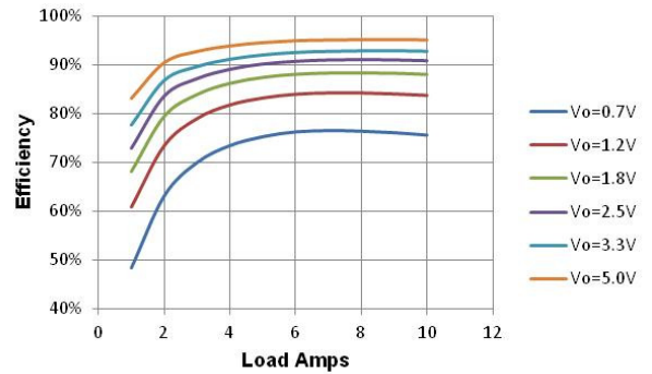
Figure 4 Efficiency vs. Load, V_{in} = 8\text{V} , F_{sw} = 500\text{KHz}
