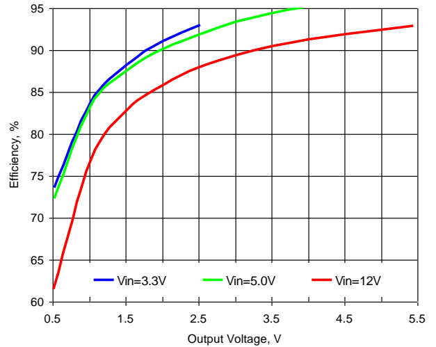
Figure 5. Efficiency vs. Output Voltage, Iout=20A, Fsw=500kHz
