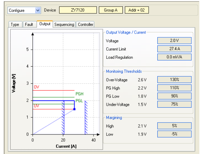
Figure 27. POL Configure Output Window
