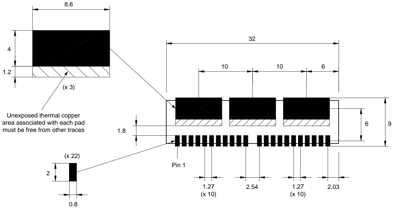
Figure 59. Recommended Pad Sizes
