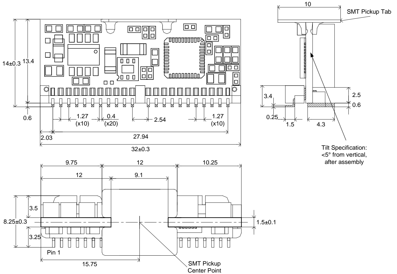
Figure 57. Mechanical Drawing
