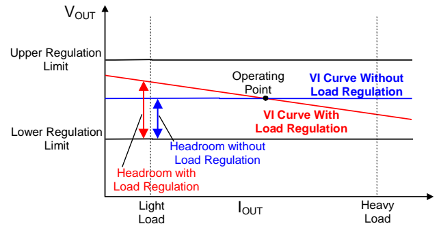
Figure 29. Concept of Optimal Voltage Positioning
