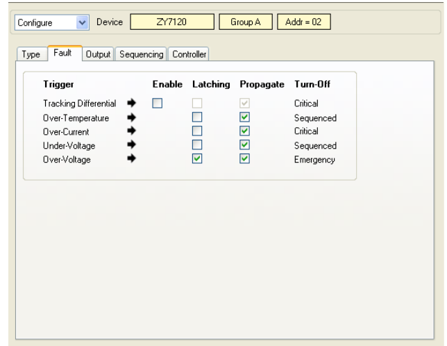
Figure 40. POL Configure Fault window
