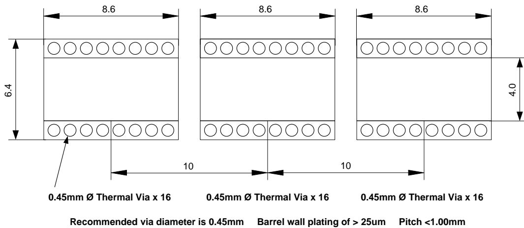
Figure 60. Recommended PCB Layout for Multilayer PCBs
