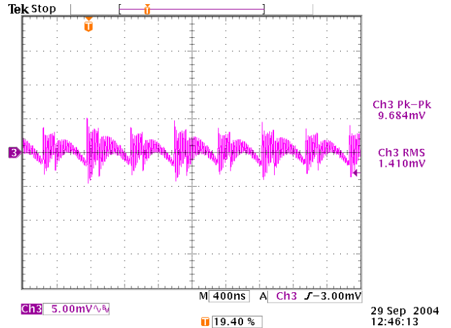
Figure 52. Output Voltage Noise, Full Load, 180° Interleave
