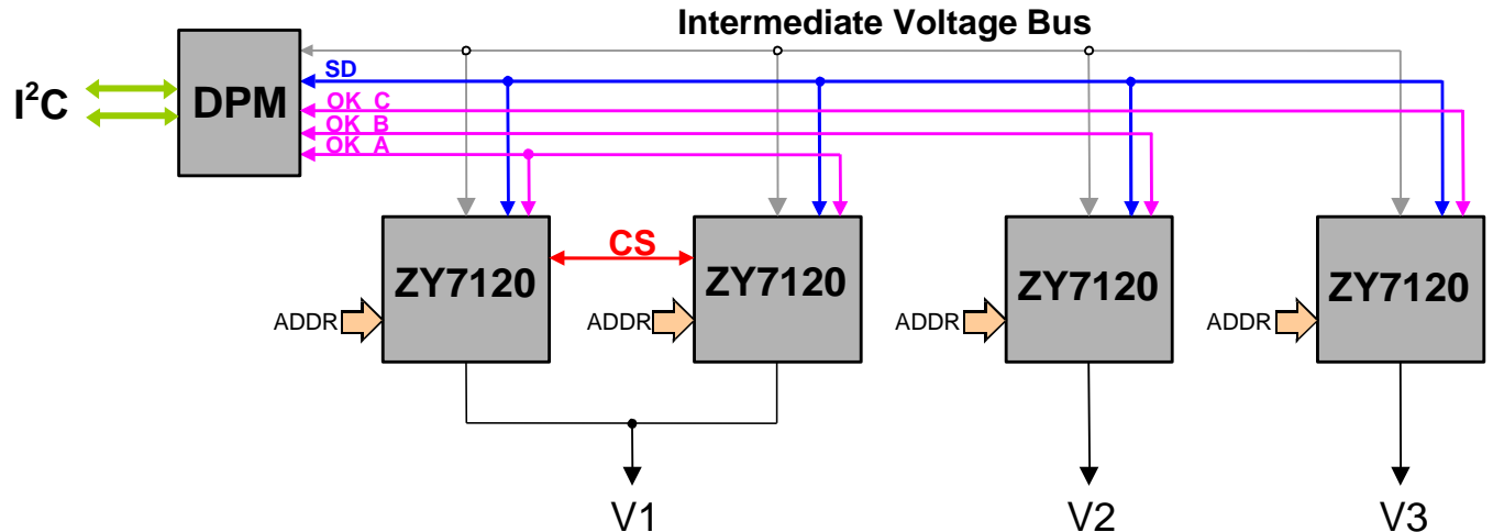
Figure 25. Block Diagram of Typical Multiple Output Application with Digital Power Manager and I 2 C Interface
