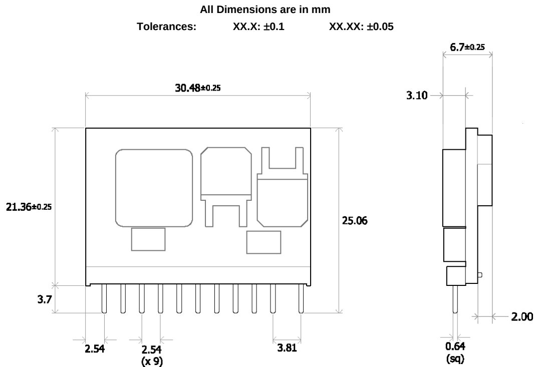
Figure 47. Mechanical Drawing
