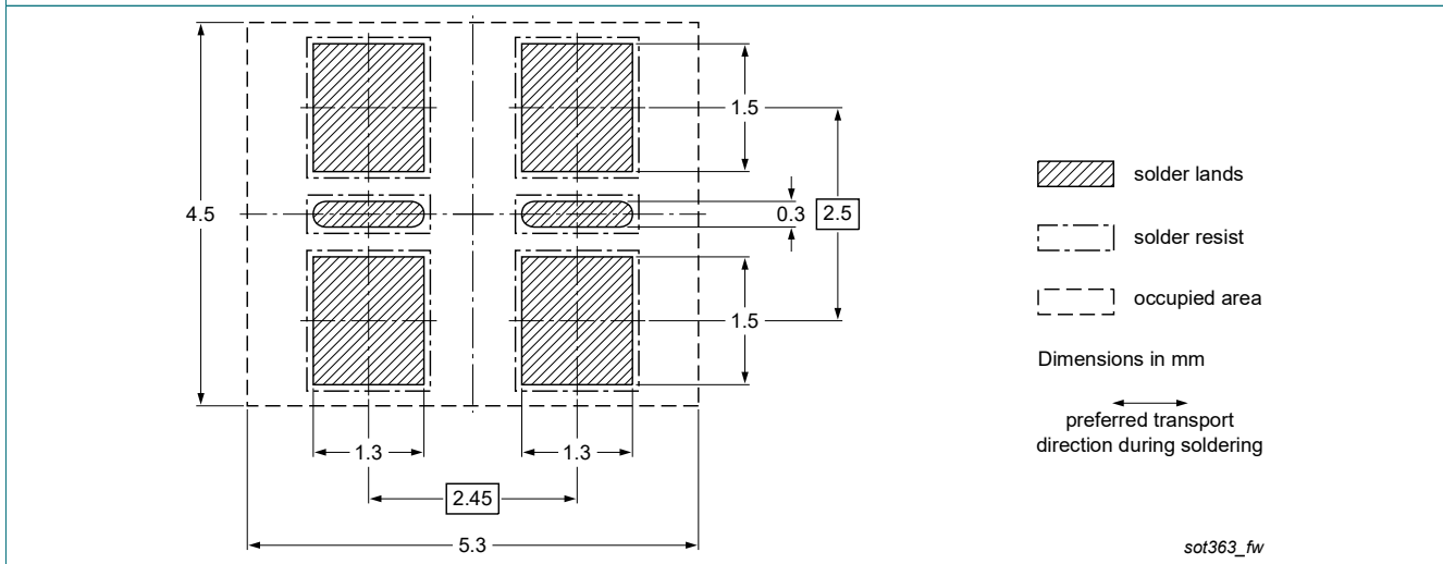
Fig. 11. Wave soldering footprint for TSSOP6 (SOT363)
