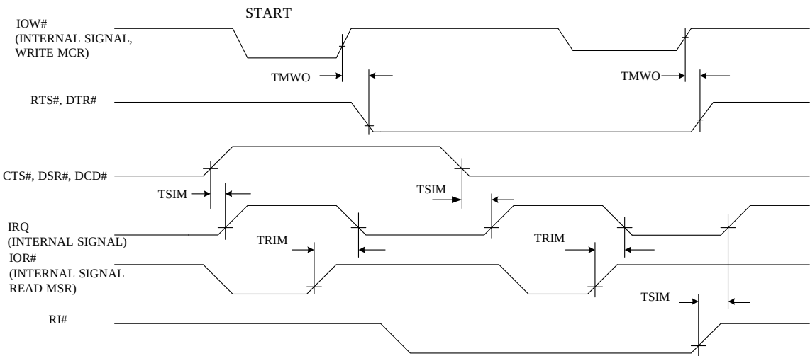
MODEM Control Timing
