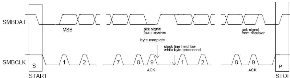
Figure 18-1 Data Transfer Format
