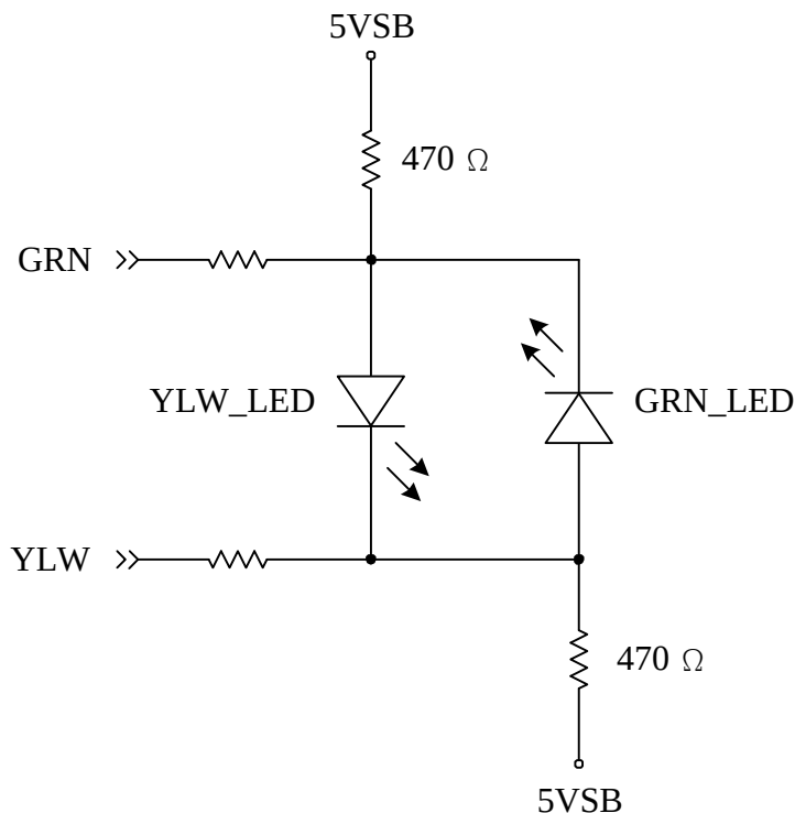
Figure 6-8 Illustration of Dual Color LED application
