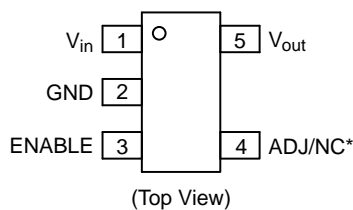
Figure 2. TSOP5
