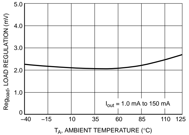
Figure 28. Load Regulation vs. Temperature
