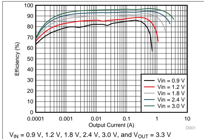
Figure 1. Load Efficiency with Different Input
