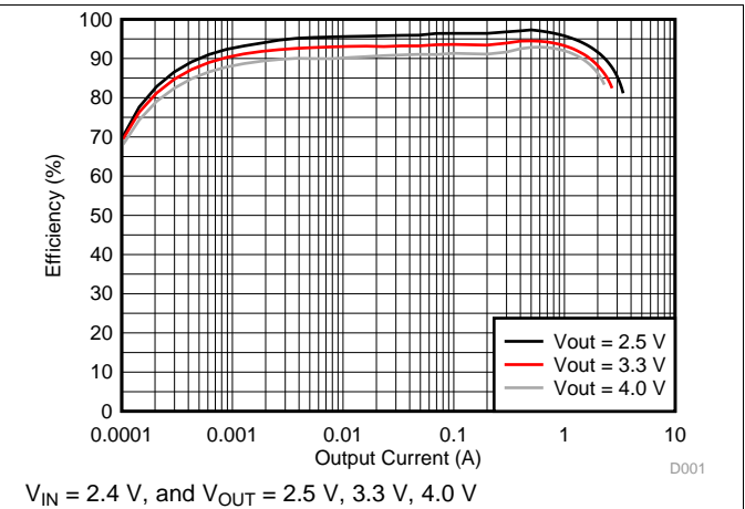
Figure 2. Load Efficiency with Different Output
