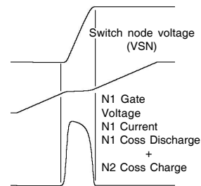
Figure 6 – Q_{OSS} Waveforms
