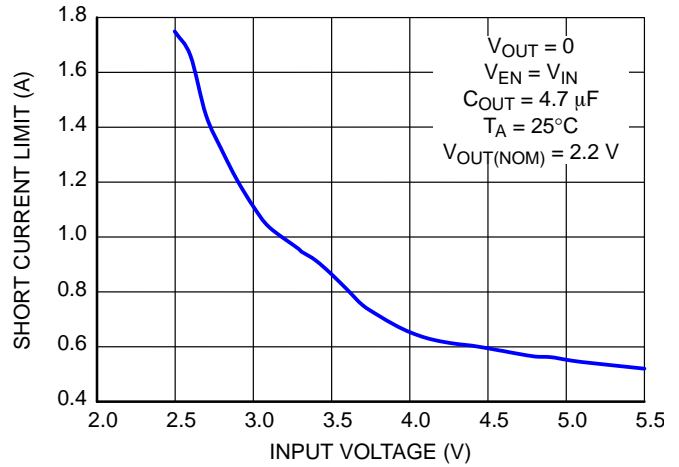
Figure 16. Short Current Limitation vs. Input Voltage
