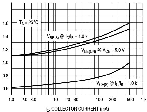
Figure 2. "ON" Voltages
