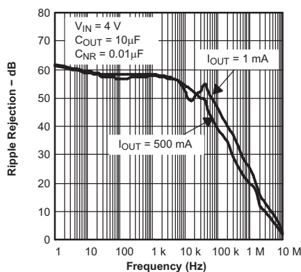
TPS79530 Ripple Rejection vs Frequency
